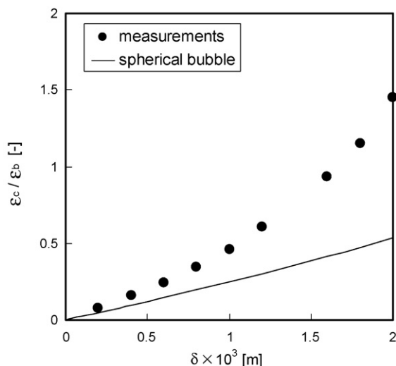
Fig. 7. Fraction of active layer around a bubble.
