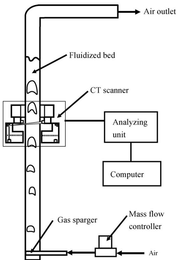
Fig. 2. Experimental equipment for the fast X-ray CT scanner/fluidized bed assembly.
