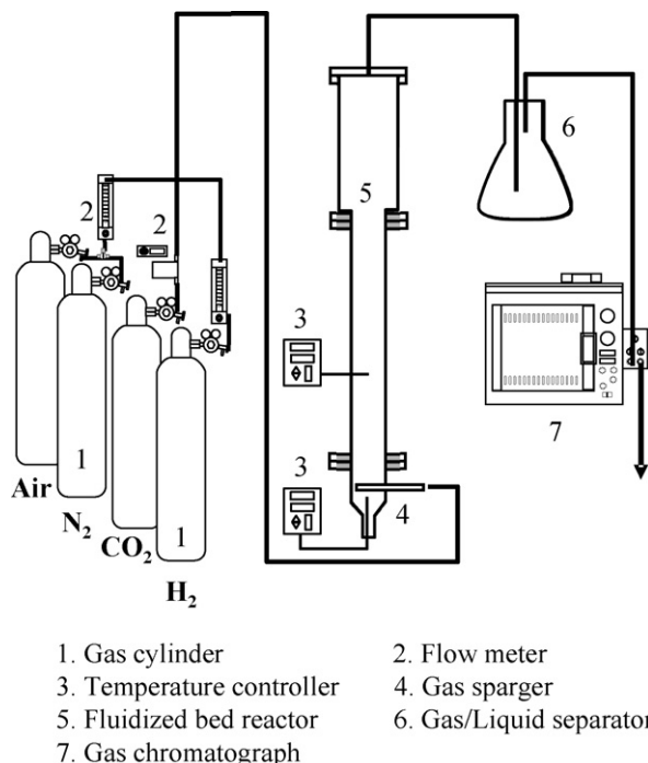
Fig. 1. Fluidized bed reactor system.
