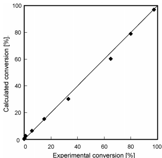
Fig. 5. The comparison of experimental conversion with the calculation from a model considering only direct contact catalysts.
