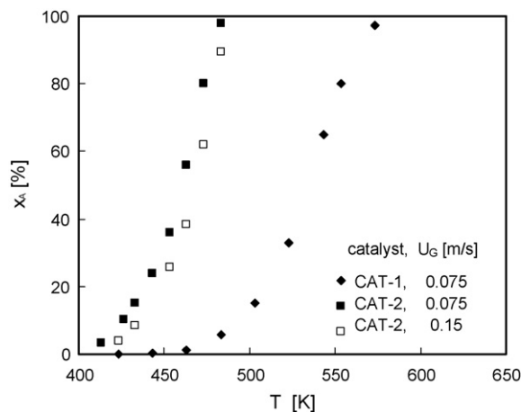
Fig. 3. The effect of reaction temperature on the conversion of carbon dioxide.
